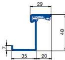
Eckzarge
